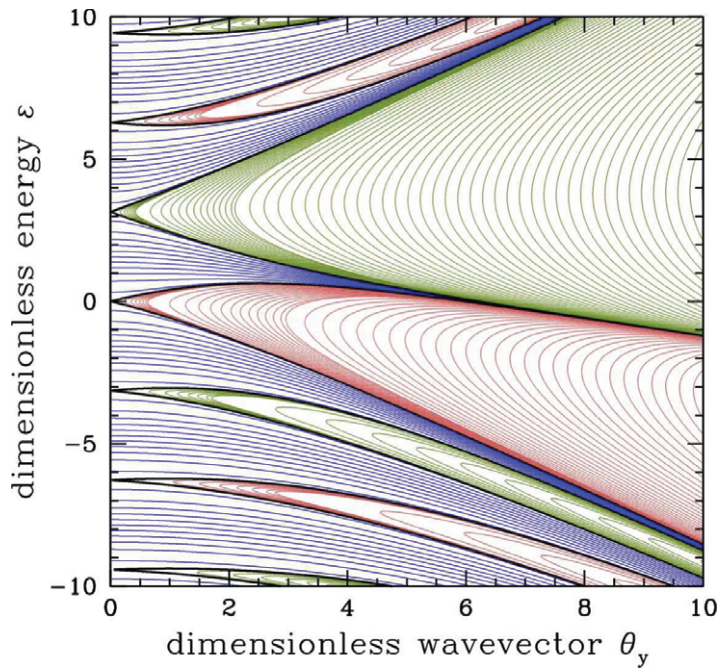
Figure 4. Contour plot of T = \text{Tr}(\Lambda) in the d_2 \rightarrow 0 limit with \Omega_0 \equiv -V_2 d_2 / \hbar v_F = \frac{3}{5}\pi held constant.
