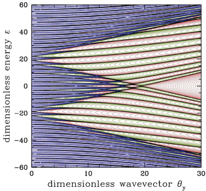
Figure 3. Contour plot of T = \text{Tr}(\Lambda) for \omega_0 = \frac{13}{2}\pi and d_1 = d_2 .
